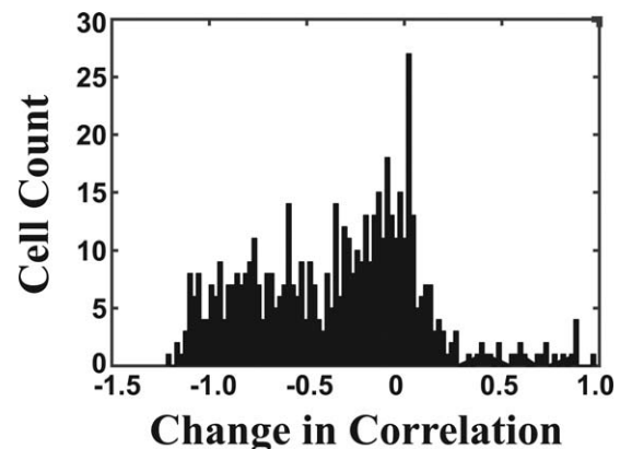
FIGURE 6. Distribution of the change in spatial correlations for repeated visits to the same context resulting from rotation of one of the firing rate maps. Data are shown for all neurons and all rotations ( 90^\circ , 180^\circ , or 270^\circ ) from the first recording day. Most correlations were similar to the original nonrotated values or were reduced (i.e., values near zero and to the left of zero).
